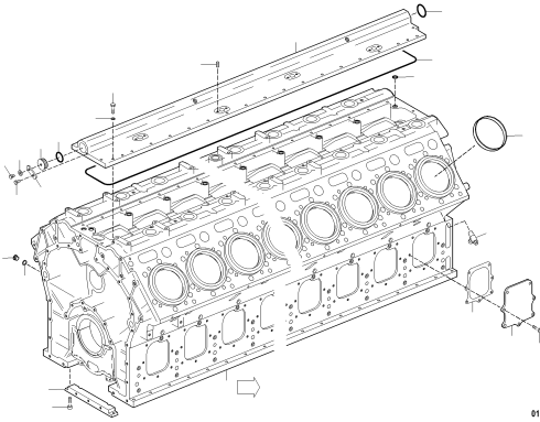
CRANKCASE UPC.06A01 2081
