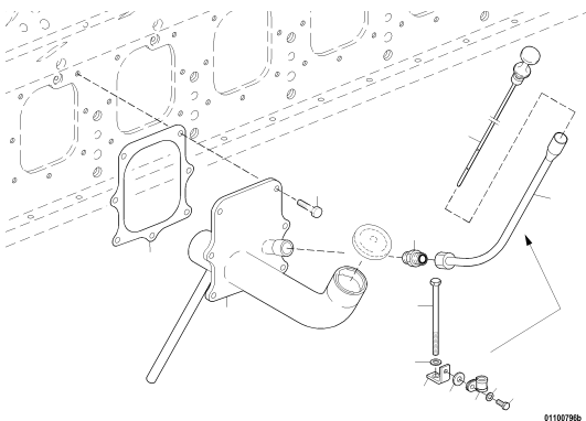
OIL FILLER NECK UPC.06G04 1388
